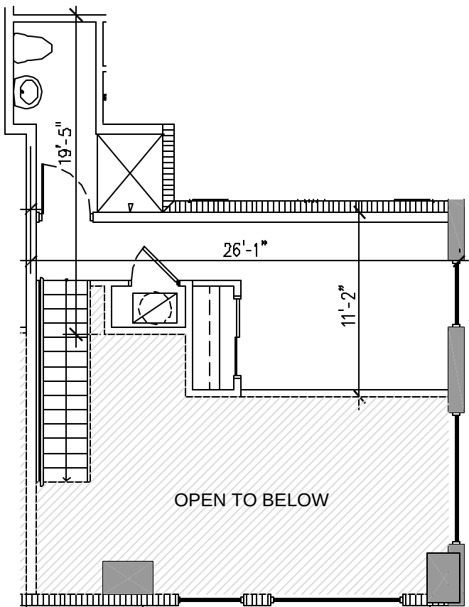
Mezzanine Level
