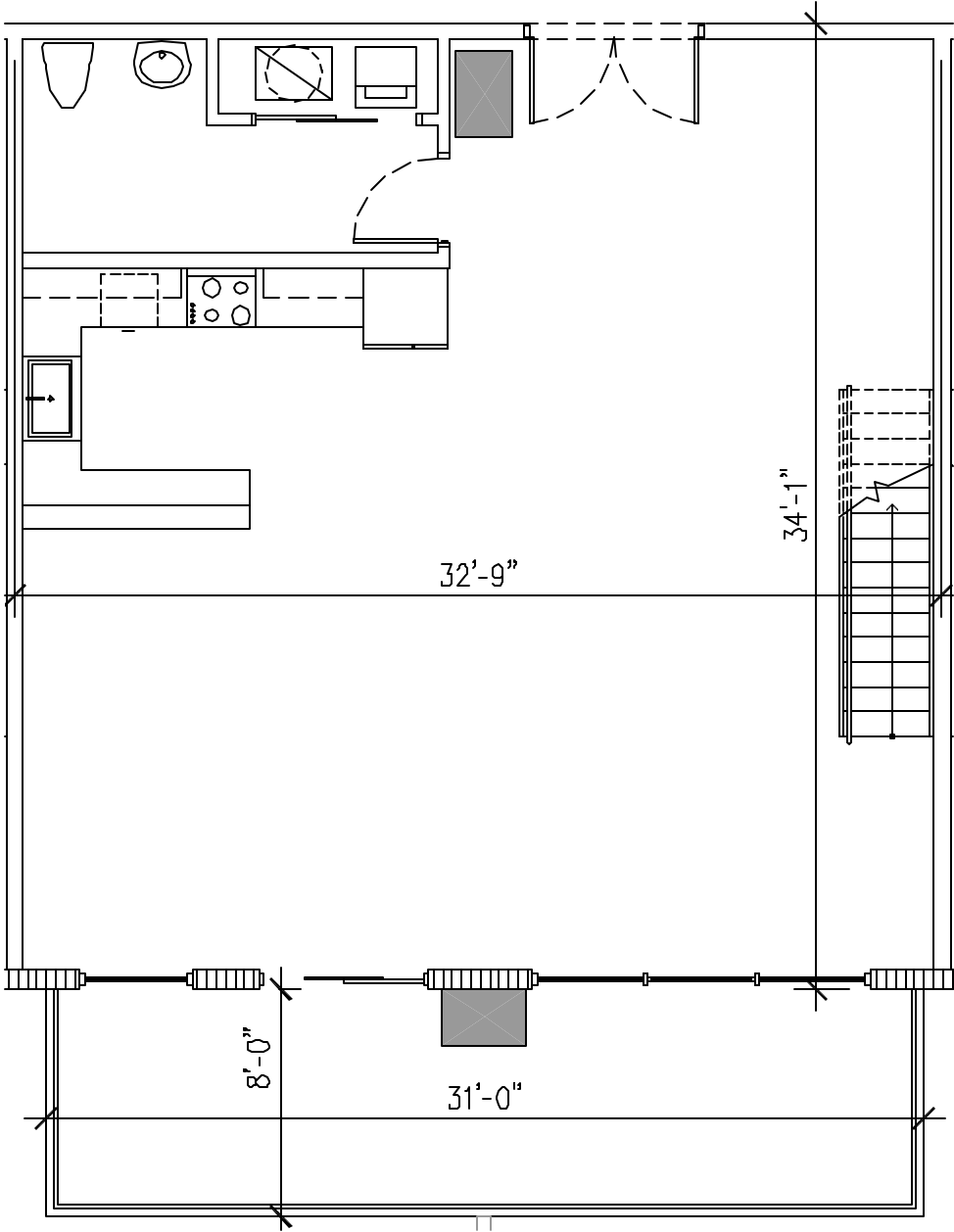
Ground Level
